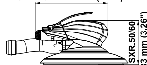
SXR.C = 133 mm (5.24")
