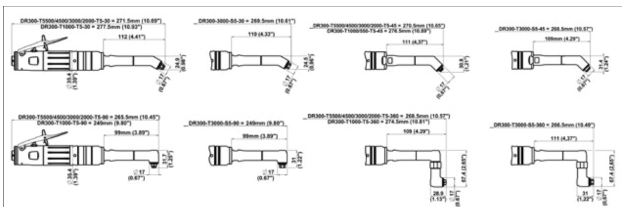
C Serie DR300-T...-T/S5-90 300 W (0.4 hp) - 1000 a 5500 rpm
